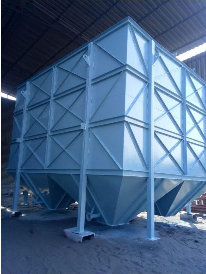
Tube settler ↑
